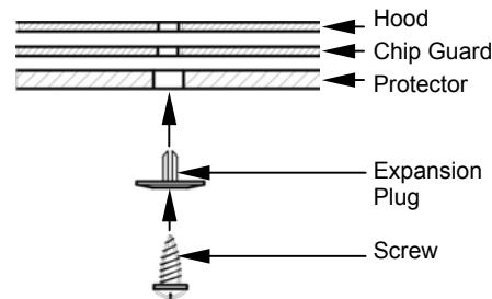
Illustration #1 : Hardware Assembly
